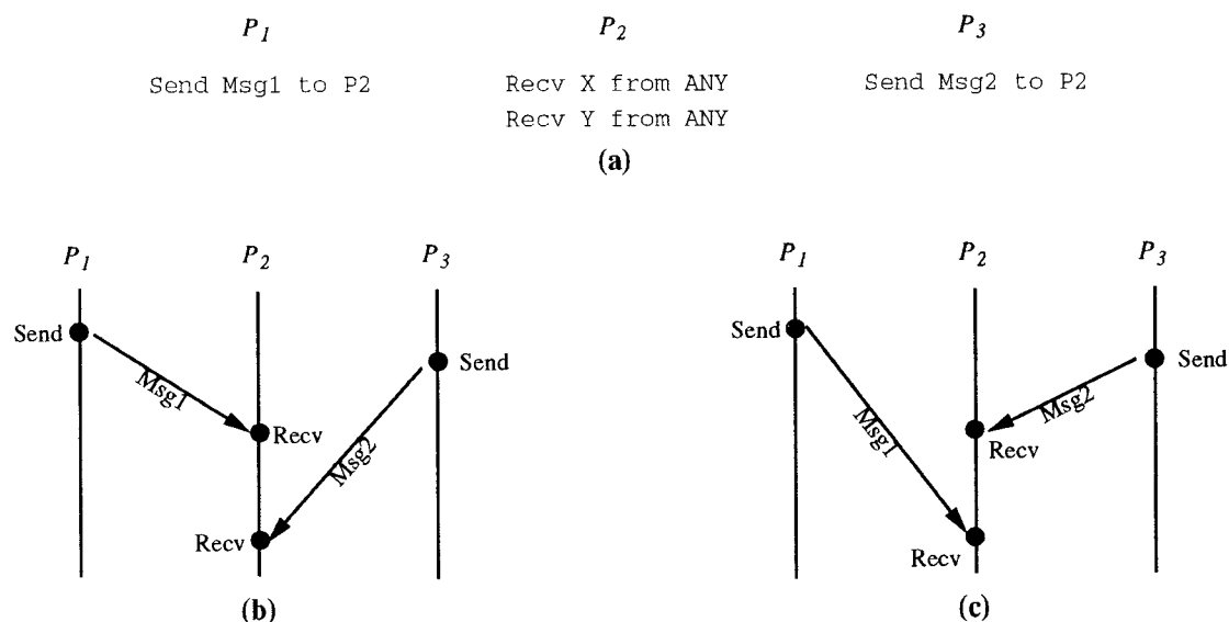
Figure 1. (a) example message-passing program, and (b),(c) two possible executions
