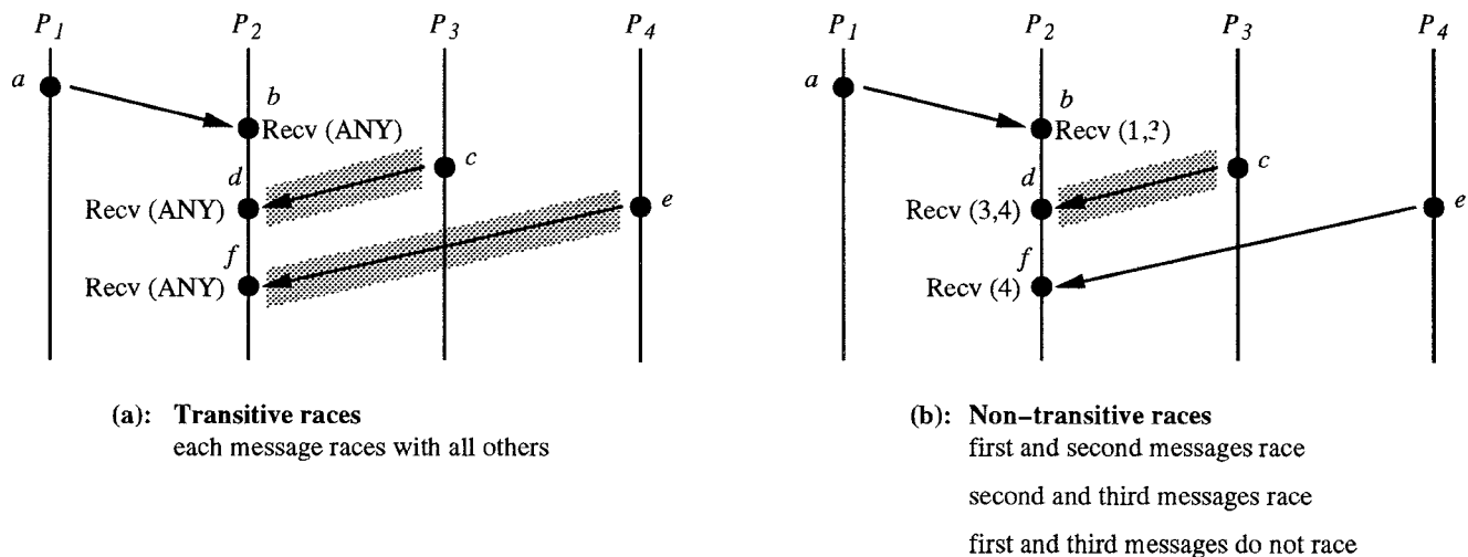
Figure 4. (a) Transitive races, (b) non-transitive races: shaded messages show the optimal trace (tracing algorithm would trace the last two messages)
