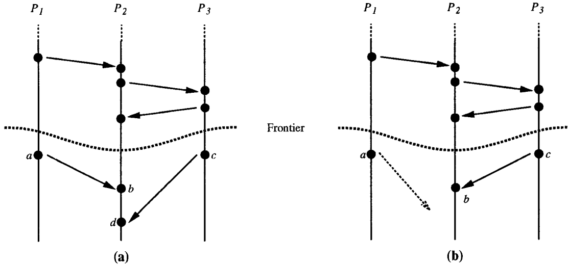
Figure 2. (a) one possible frontier, (b) the message from c could have been received by b
